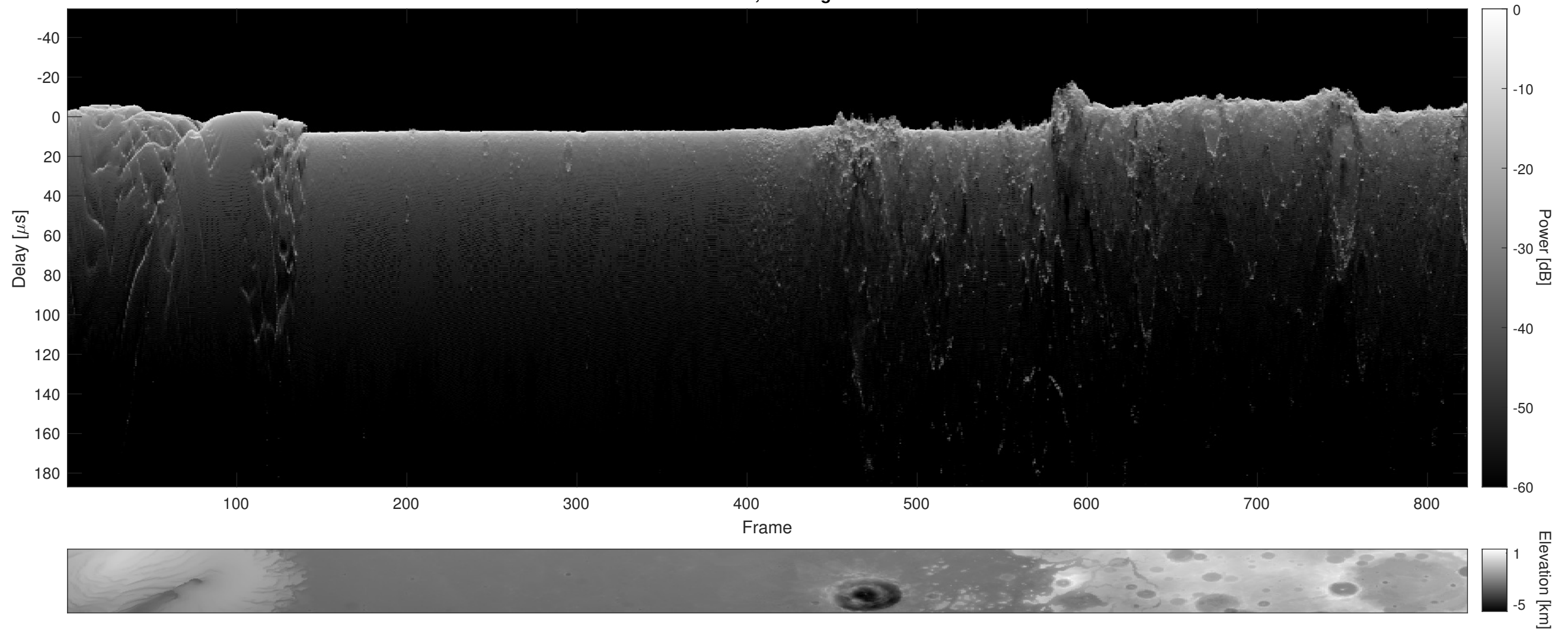
Orbit 9505, Cluttergram
