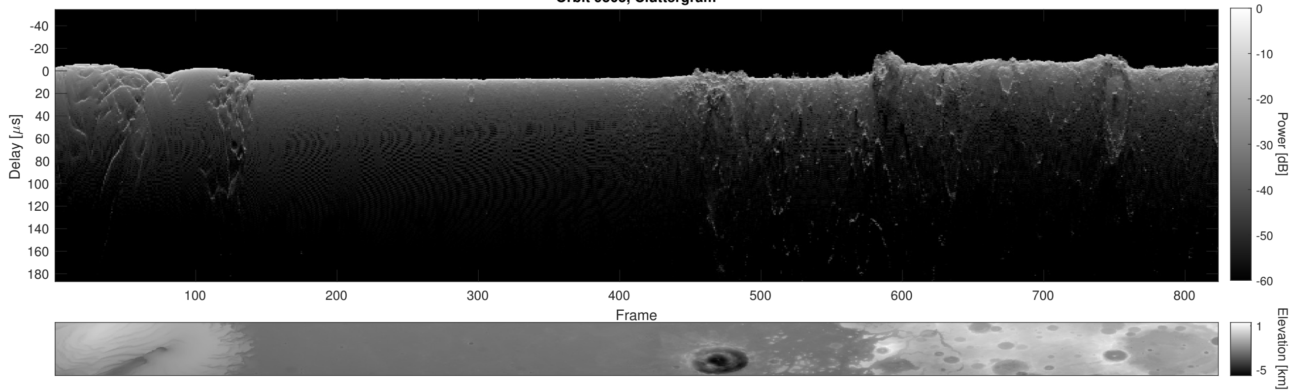
Orbit 9505, Cluttergram
