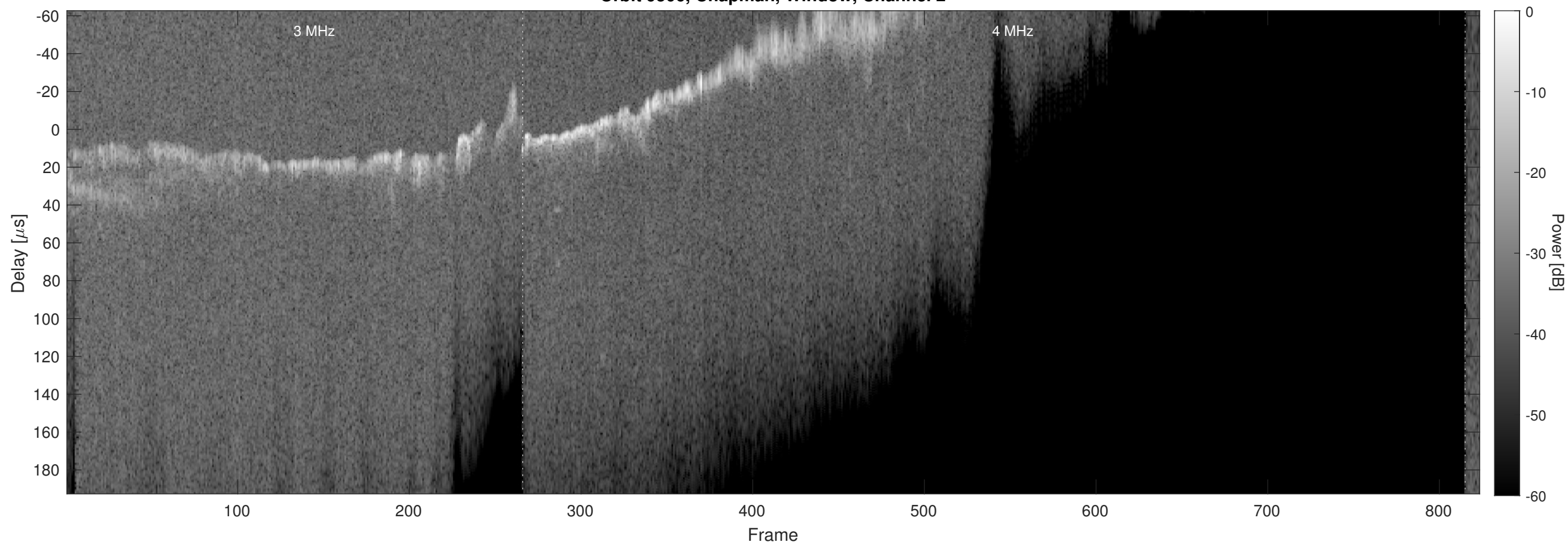
Orbit 9506, Chapman, Window, Channel 2
