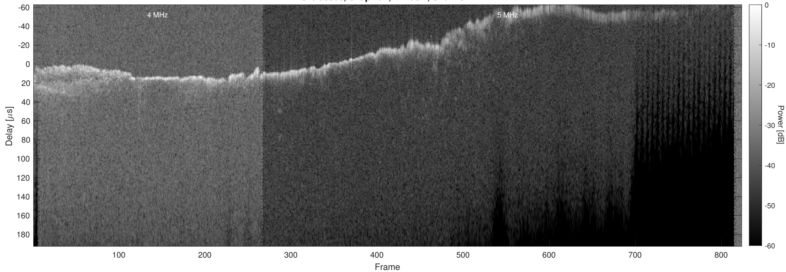
Orbit 9506, Chapman, Window, Channel 2
