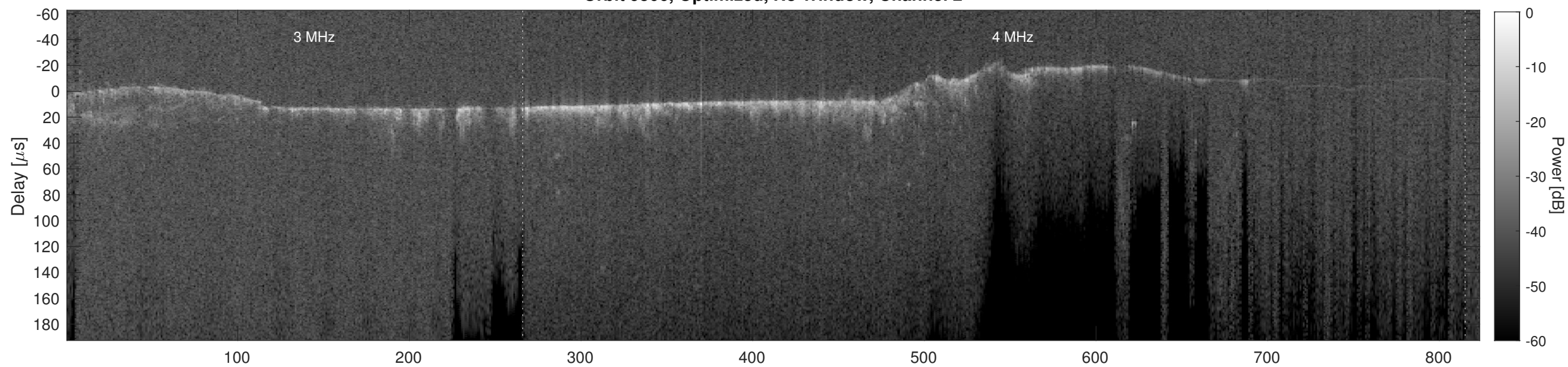
Orbit 9506, Cluttergram
