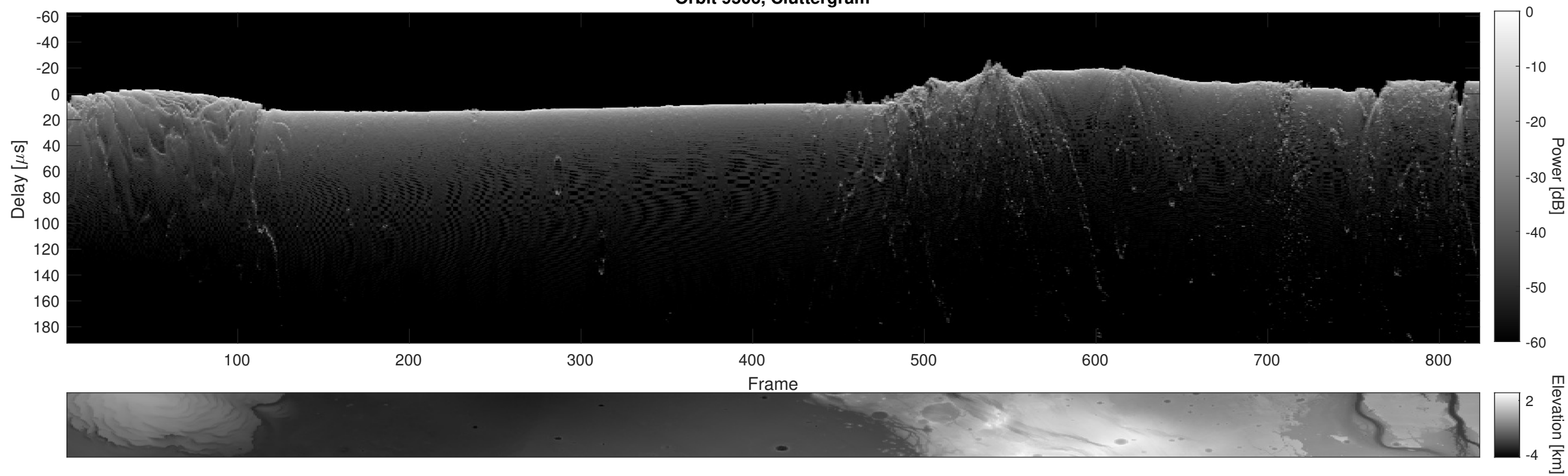
Orbit 9506, Cluttergram
