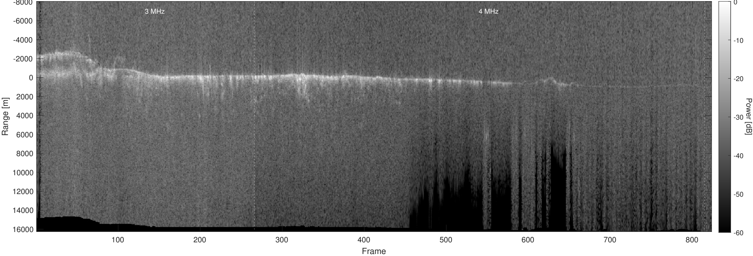
Orbit 9507, Optimized, No Window, Depth-Corrected, Channel 2
