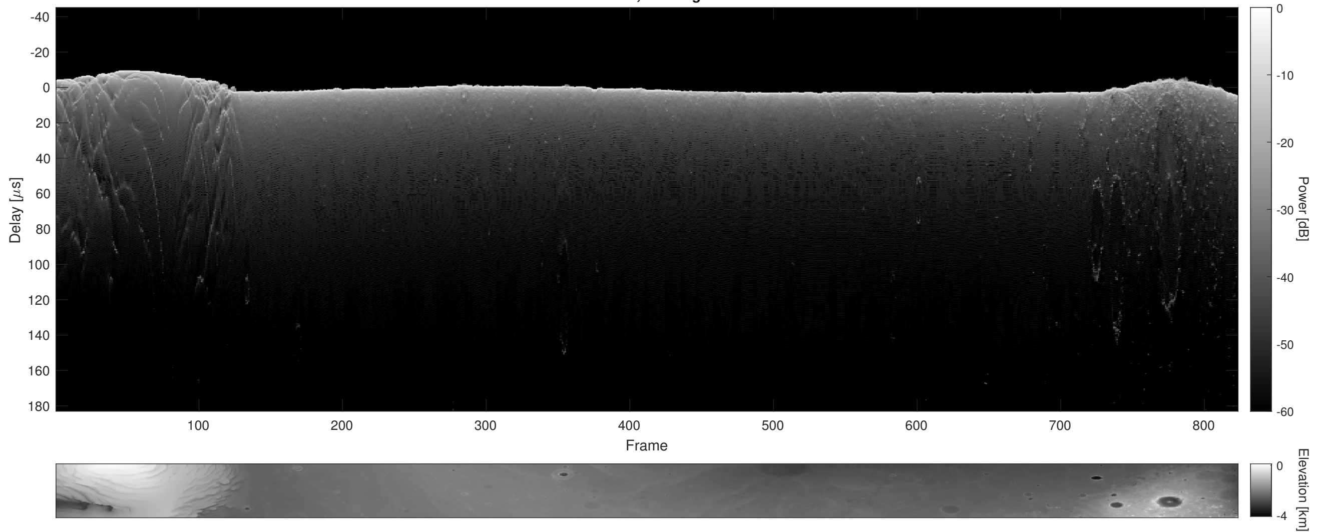
Orbit 9508, Cluttergram
