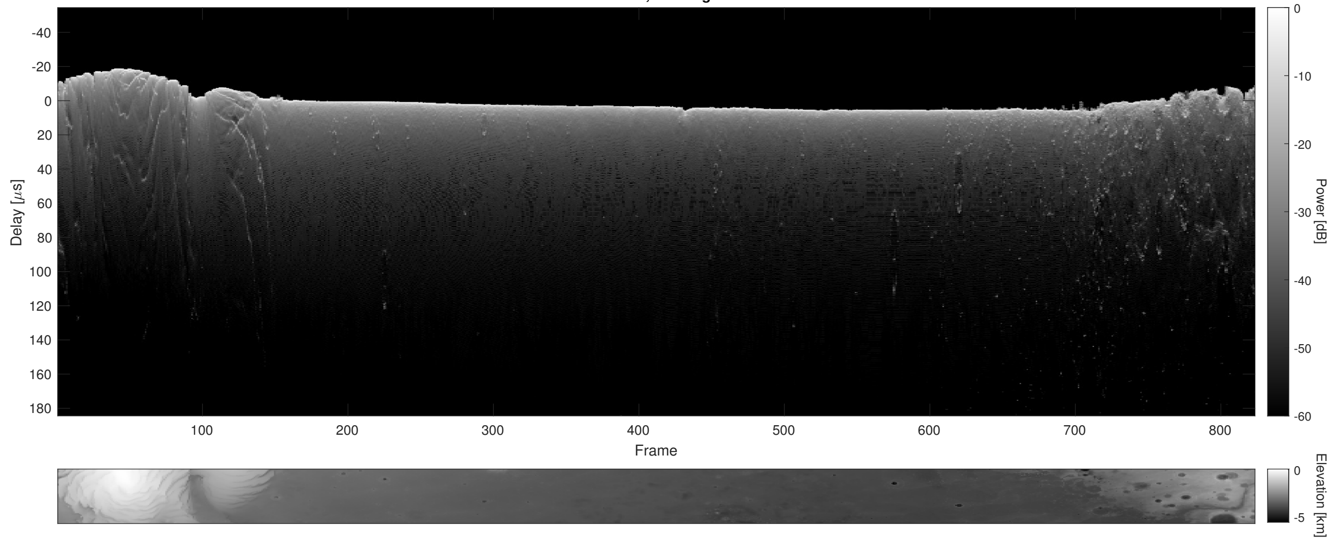
Orbit 9509, Cluttergram
