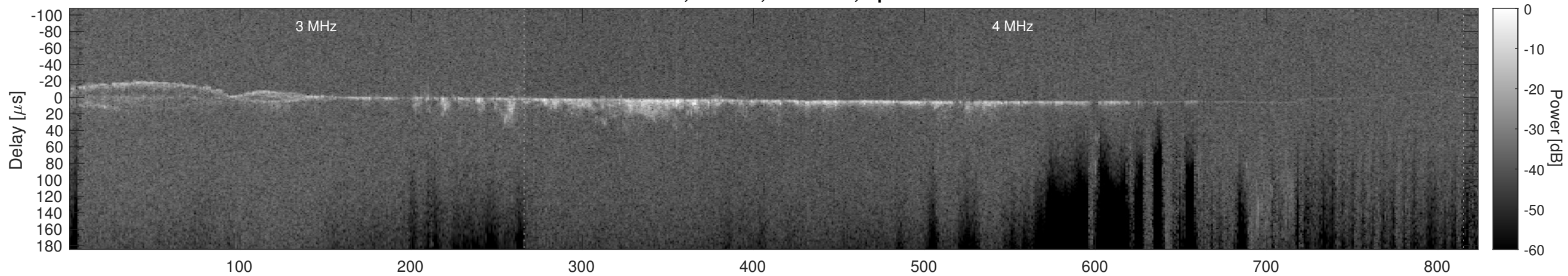
Orbit 9509, Cluttergram
