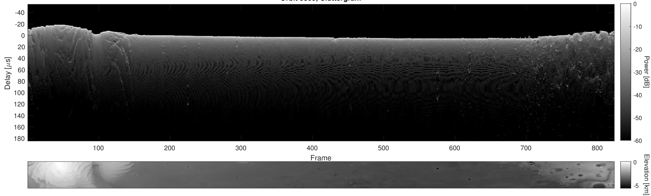
Orbit 9509, Cluttergram
