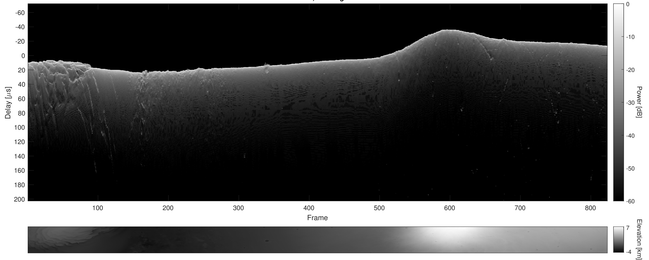
Orbit 9510, Cluttergram
