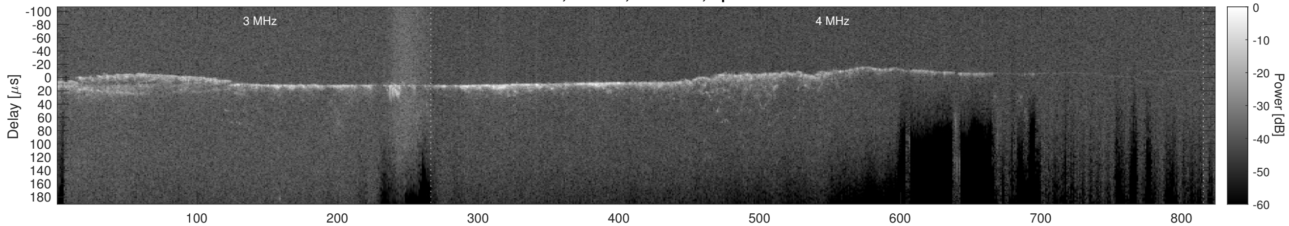
Orbit 9513, Cluttergram
