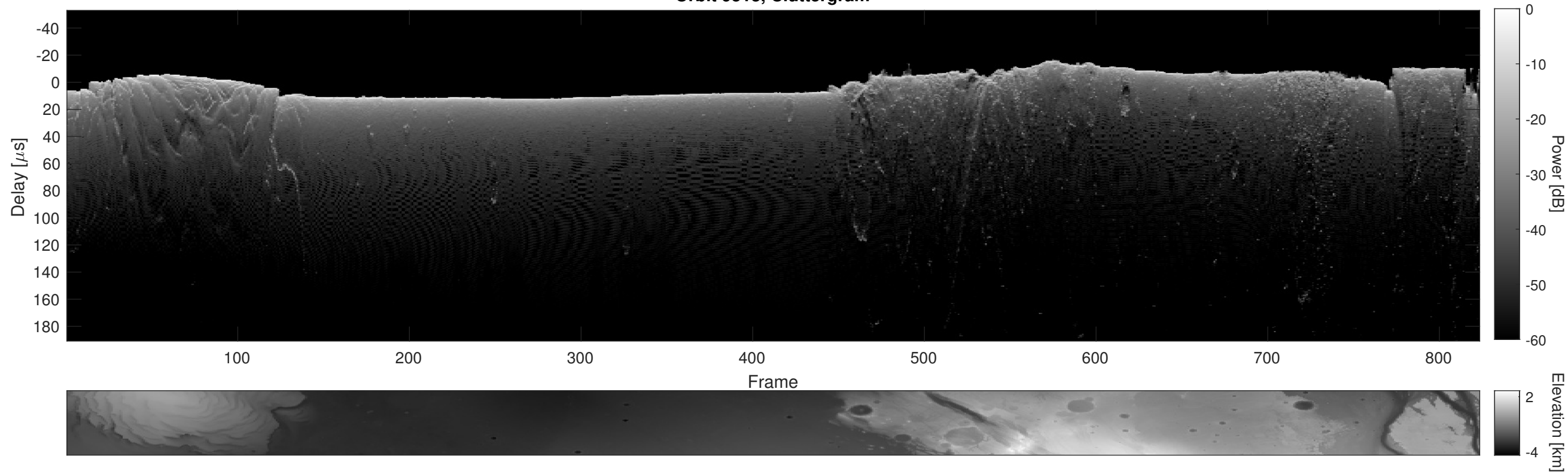
Orbit 9513, Cluttergram
