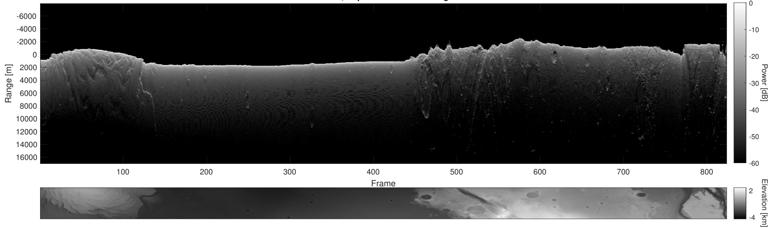
Orbit 9513, Depth-Corrected Cluttergram
