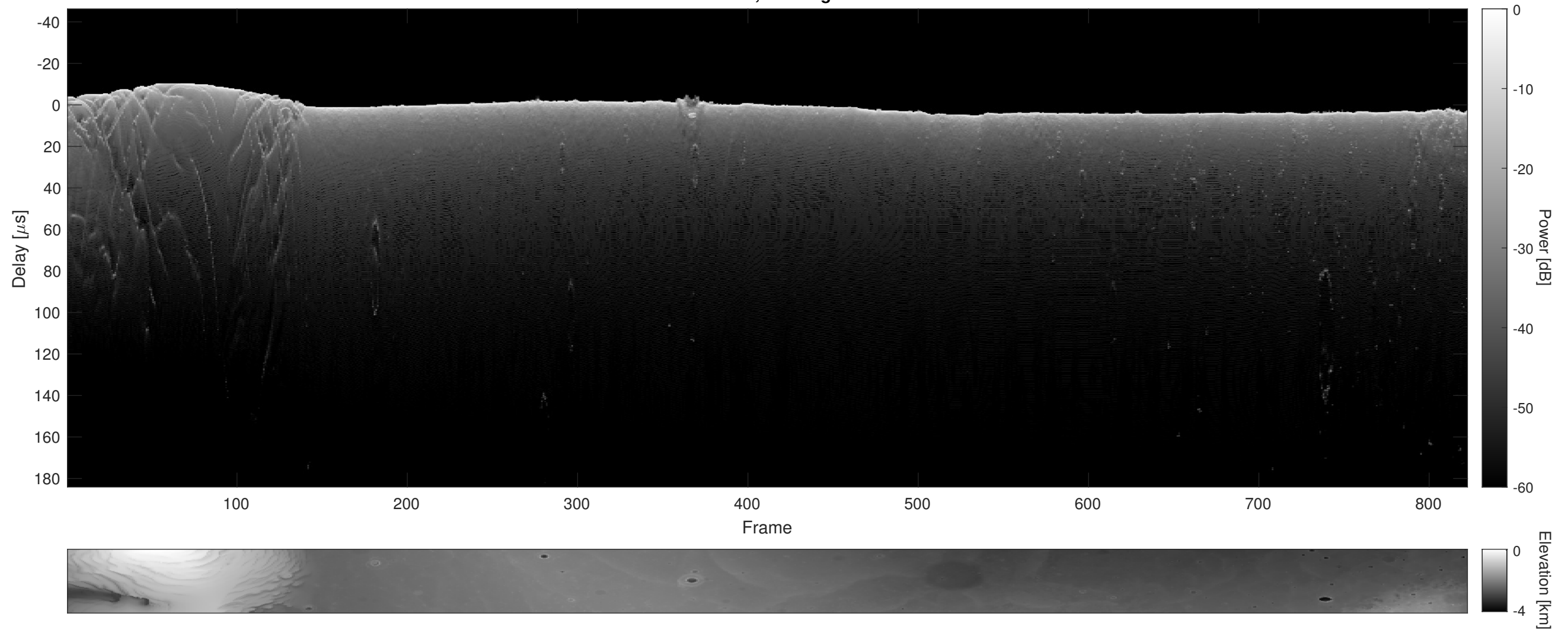
Orbit 9515, Cluttergram
