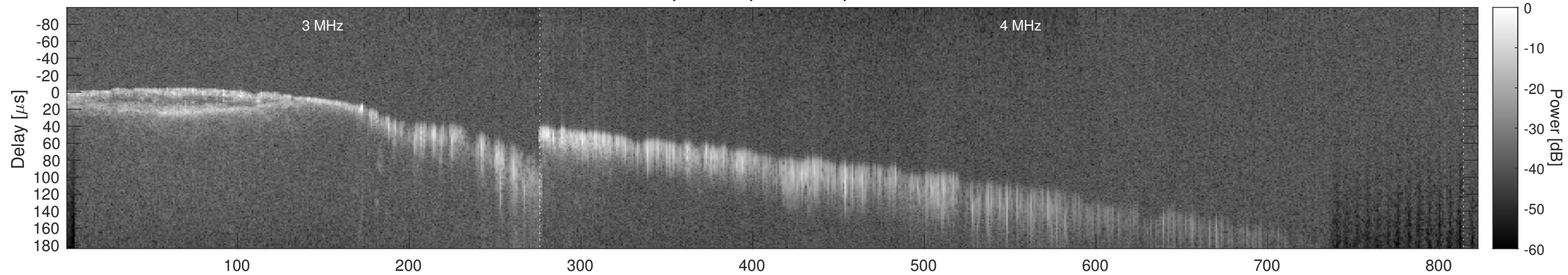
Orbit 9515, Window, Channel 2, Chapman
