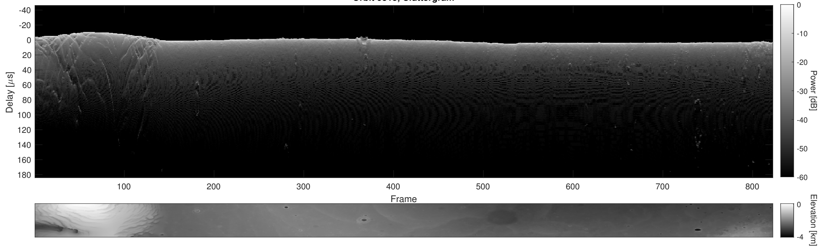
Orbit 9515, Cluttergram
