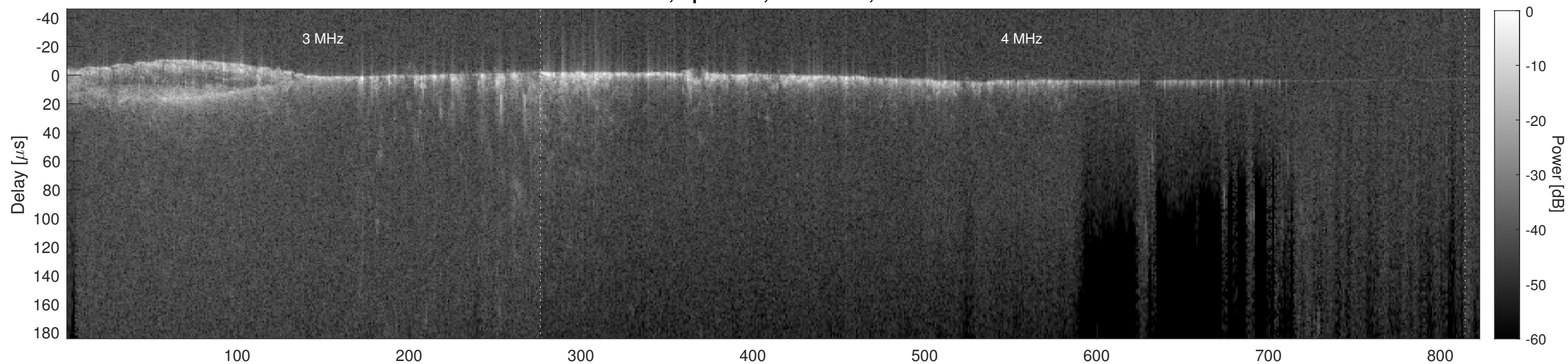
Orbit 9515, Cluttergram
