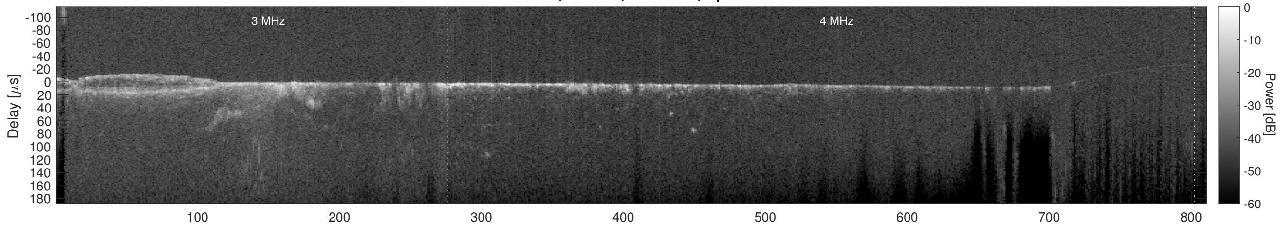
Orbit 9518, Cluttergram
