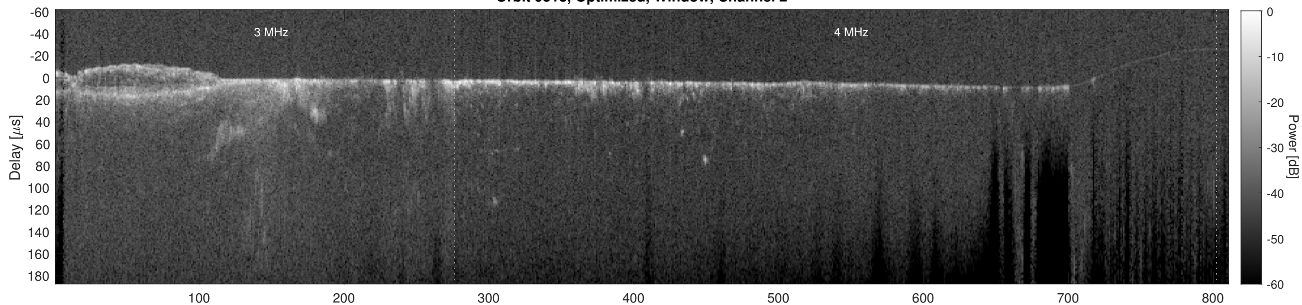
Orbit 9518, Cluttergram
