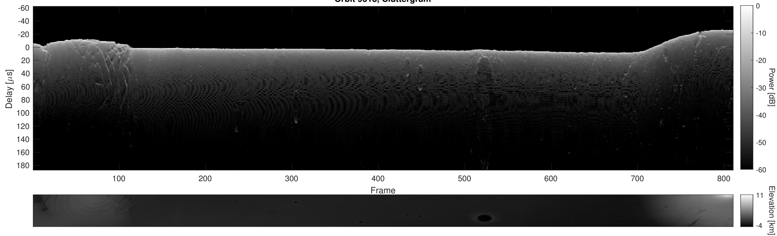
Orbit 9518, Cluttergram
