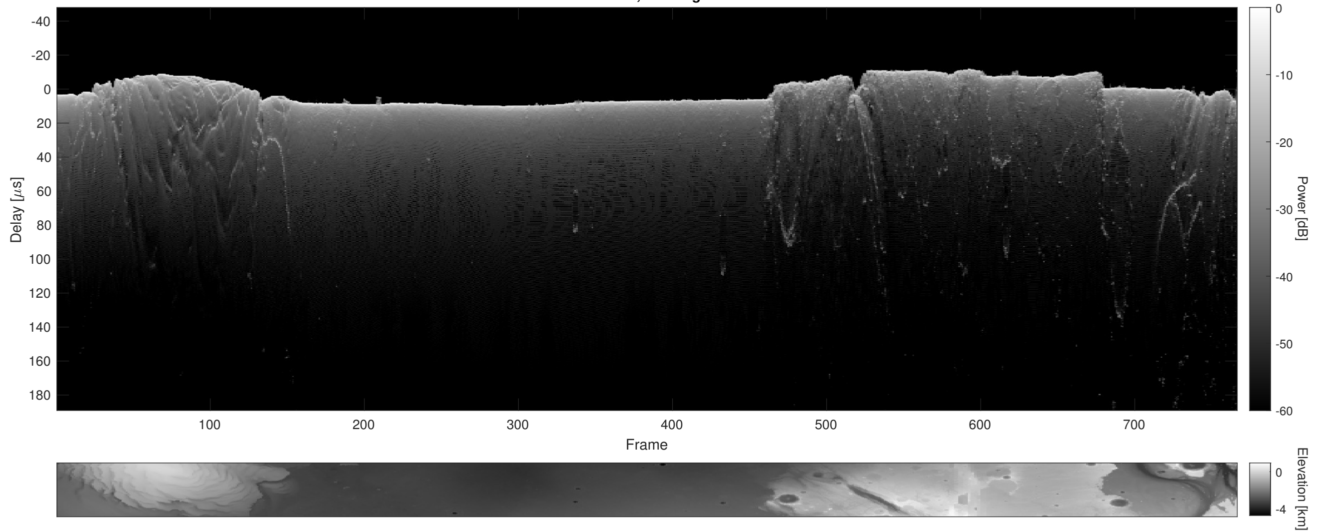
Orbit 9520, Cluttergram
