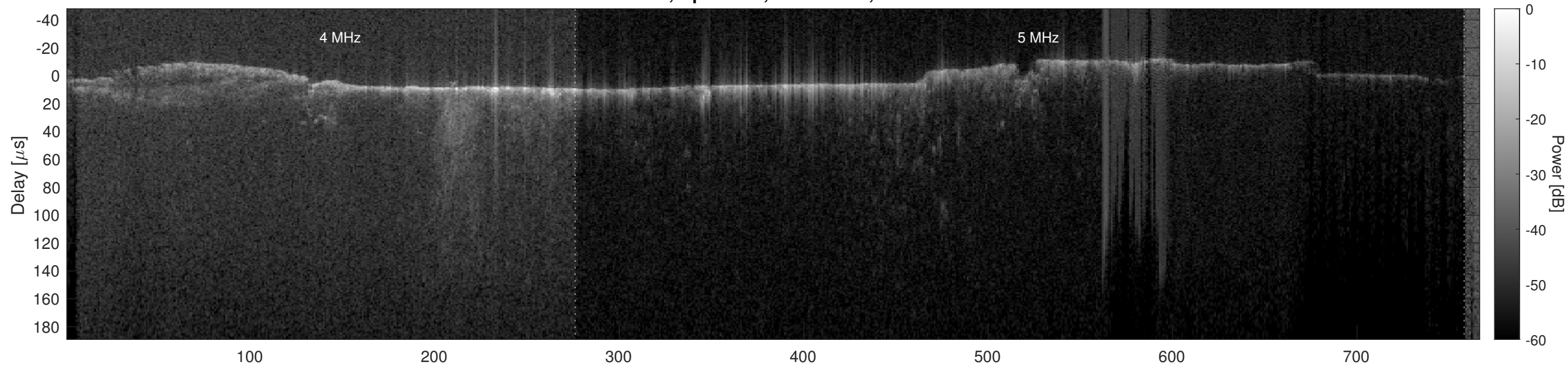
Orbit 9520, Optimized, No Window, Channel 2
