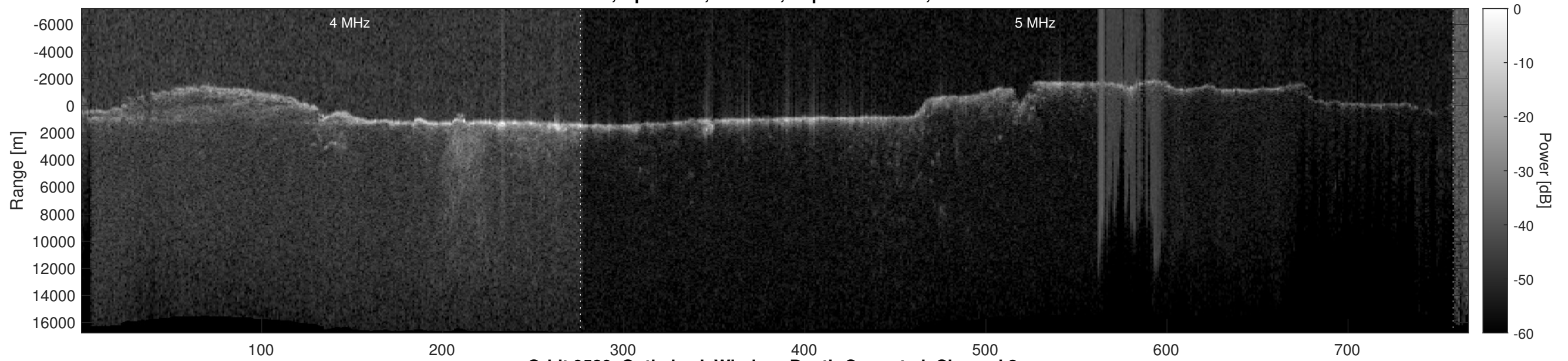
Orbit 9520, Optimized, Window, Depth-Corrected, Channel 2
