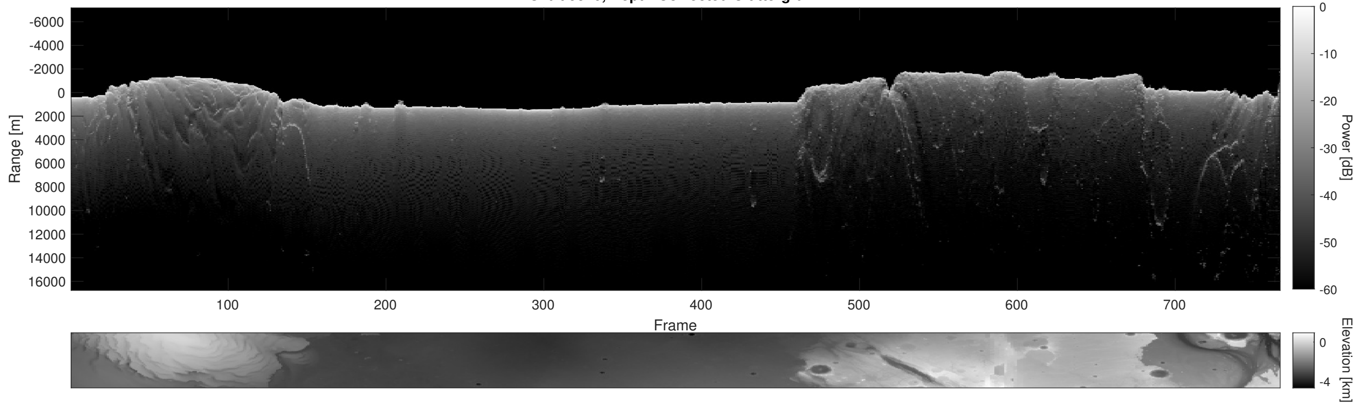
Orbit 9520, Depth-Corrected Cluttergram
