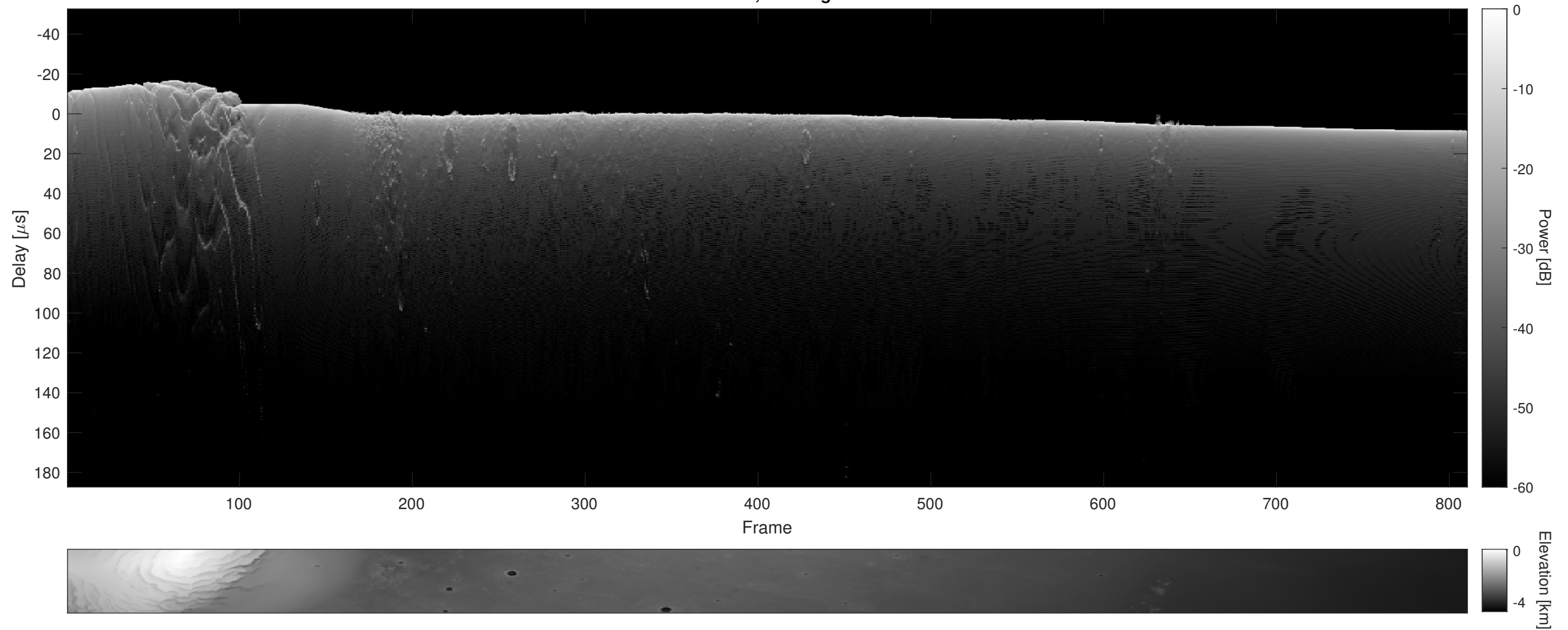
Orbit 9521, Cluttergram
