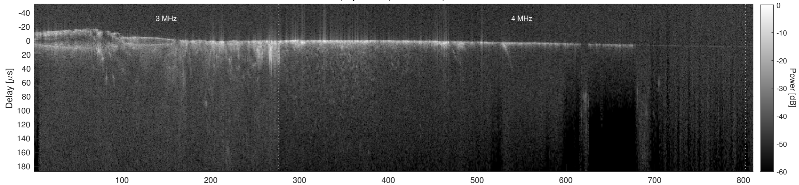
Orbit 9521, Cluttergram
