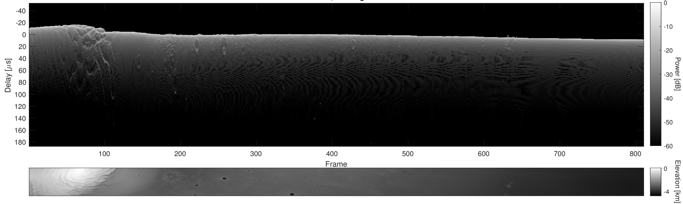
Orbit 9521, Cluttergram
