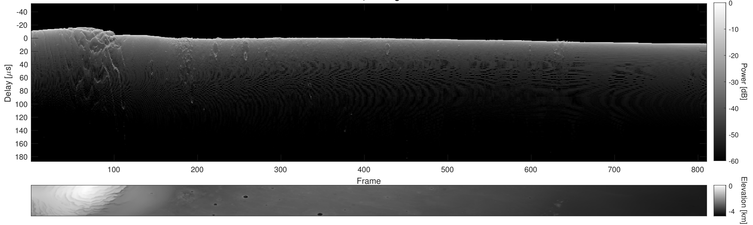
Orbit 9521, Cluttergram
