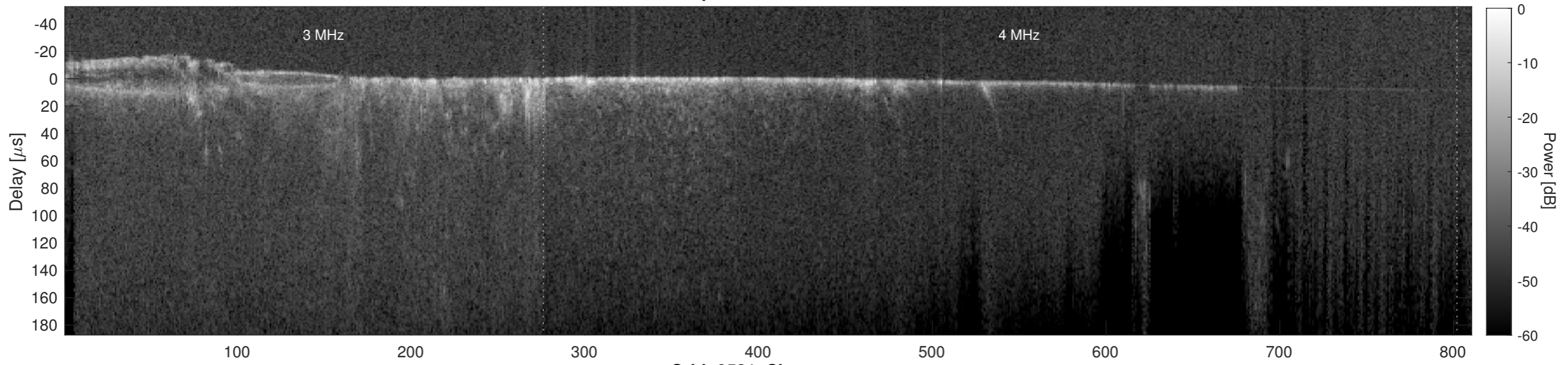
Orbit 9521, Cluttergram
