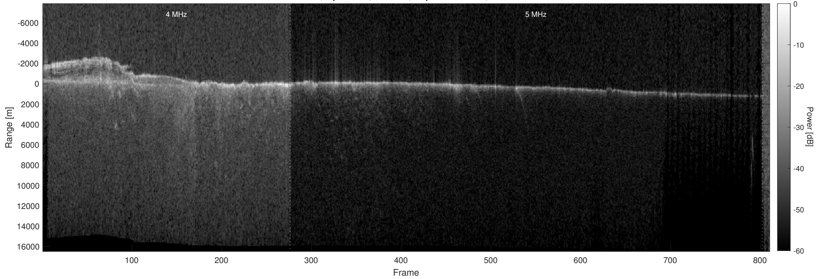
Orbit 9521, Optimized, Window, Depth-Corrected, Channel 2
