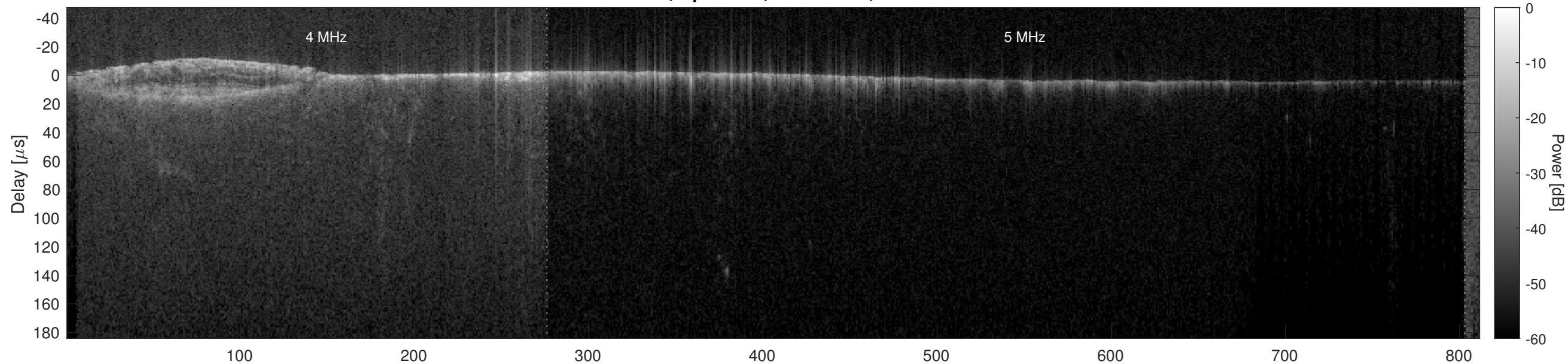
Orbit 9522, Optimized, No Window, Channel 2
