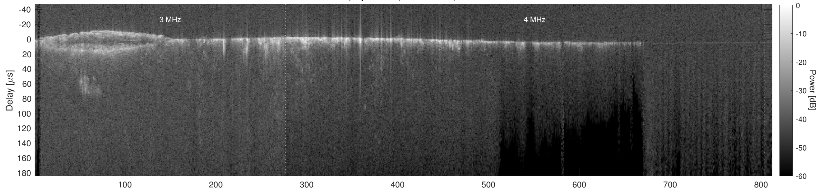
Orbit 9522, Cluttergram
