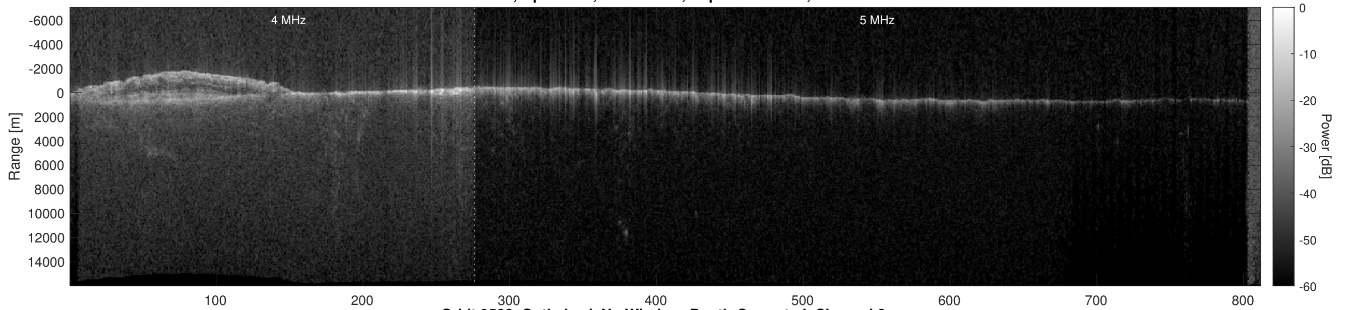
Orbit 9522, Optimized, No Window, Depth-Corrected, Channel 2
