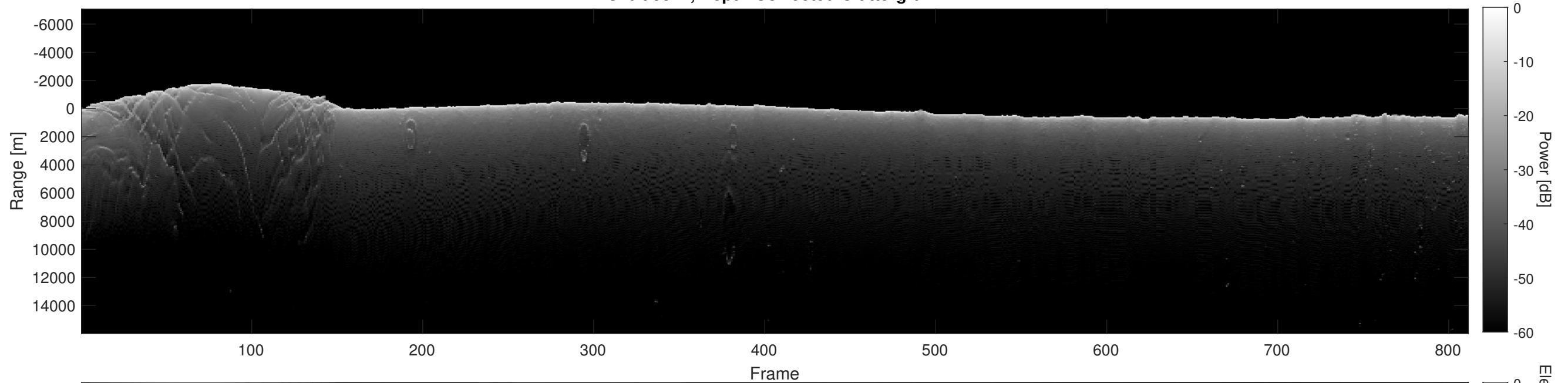
Orbit 9522, Depth-Corrected Cluttergram
