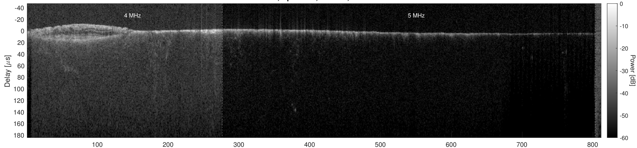
Orbit 9522, Optimized, Window, Channel 2
