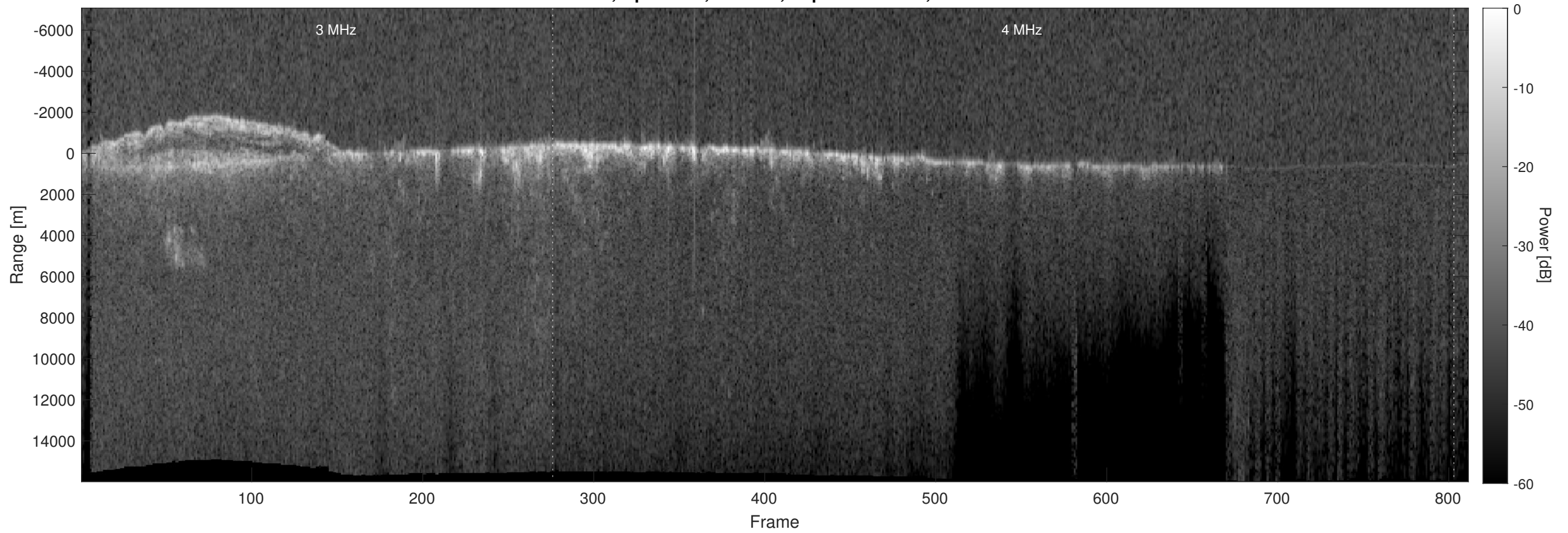
Orbit 9522, Optimized, Window, Depth-Corrected, Channel 2
