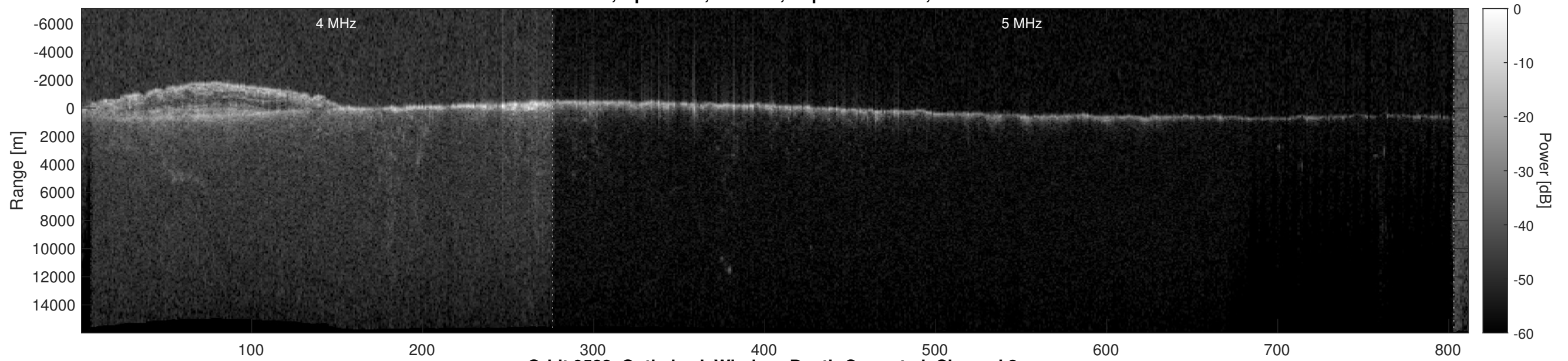
Orbit 9522, Optimized, Window, Depth-Corrected, Channel 2
