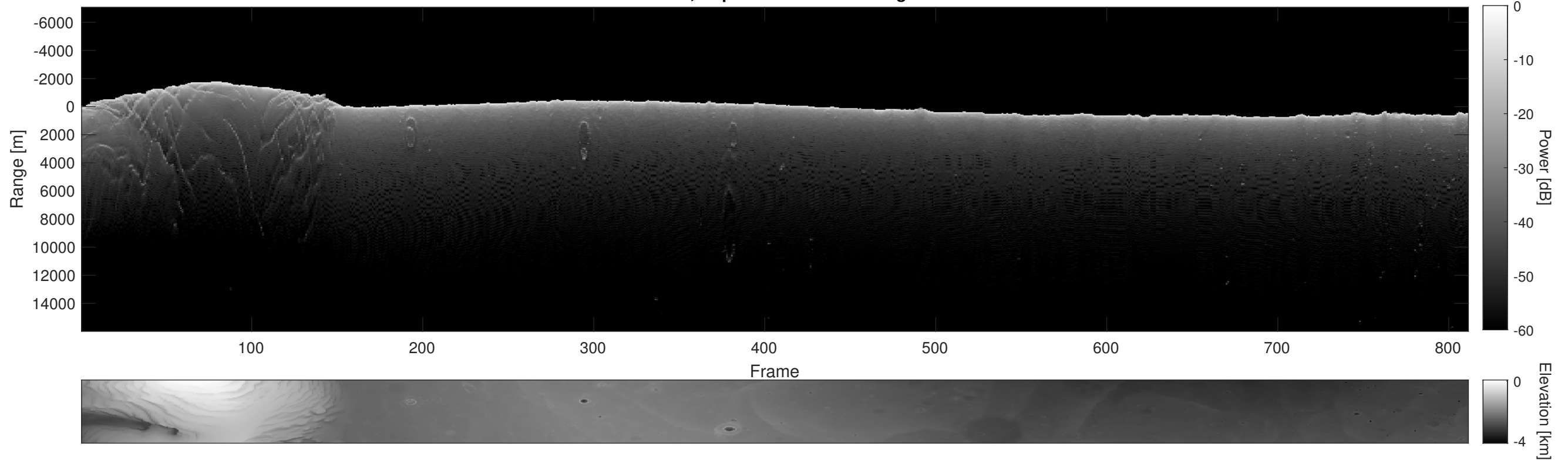
Orbit 9522, Depth-Corrected Cluttergram
