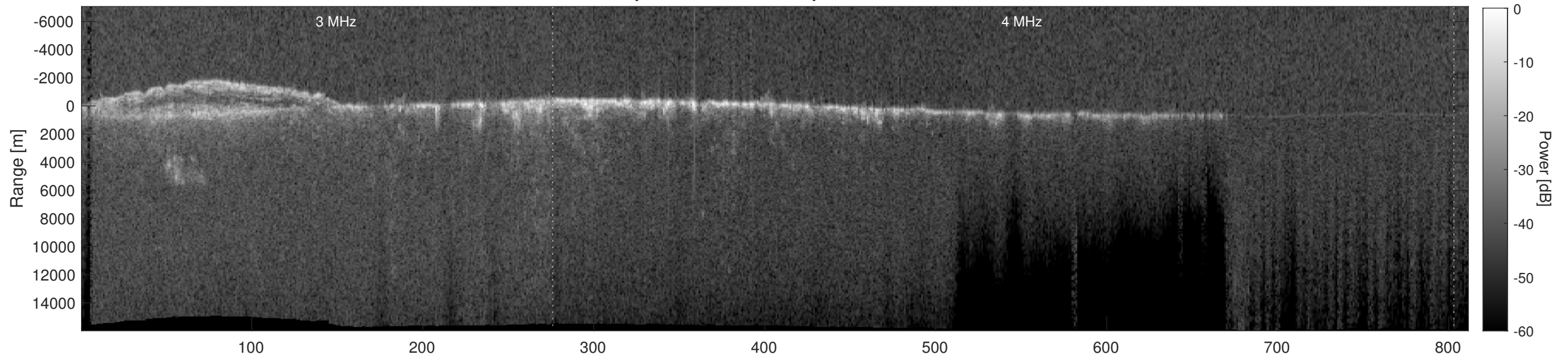
Orbit 9522, Depth-Corrected Cluttergram
