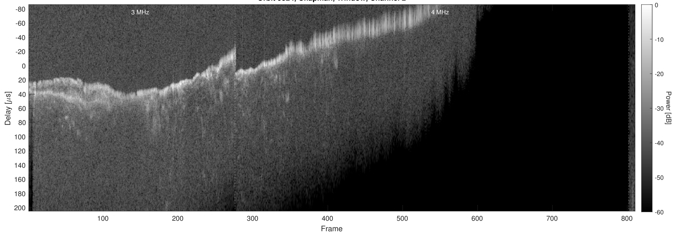
Orbit 9524, Chapman, Window, Channel 2
