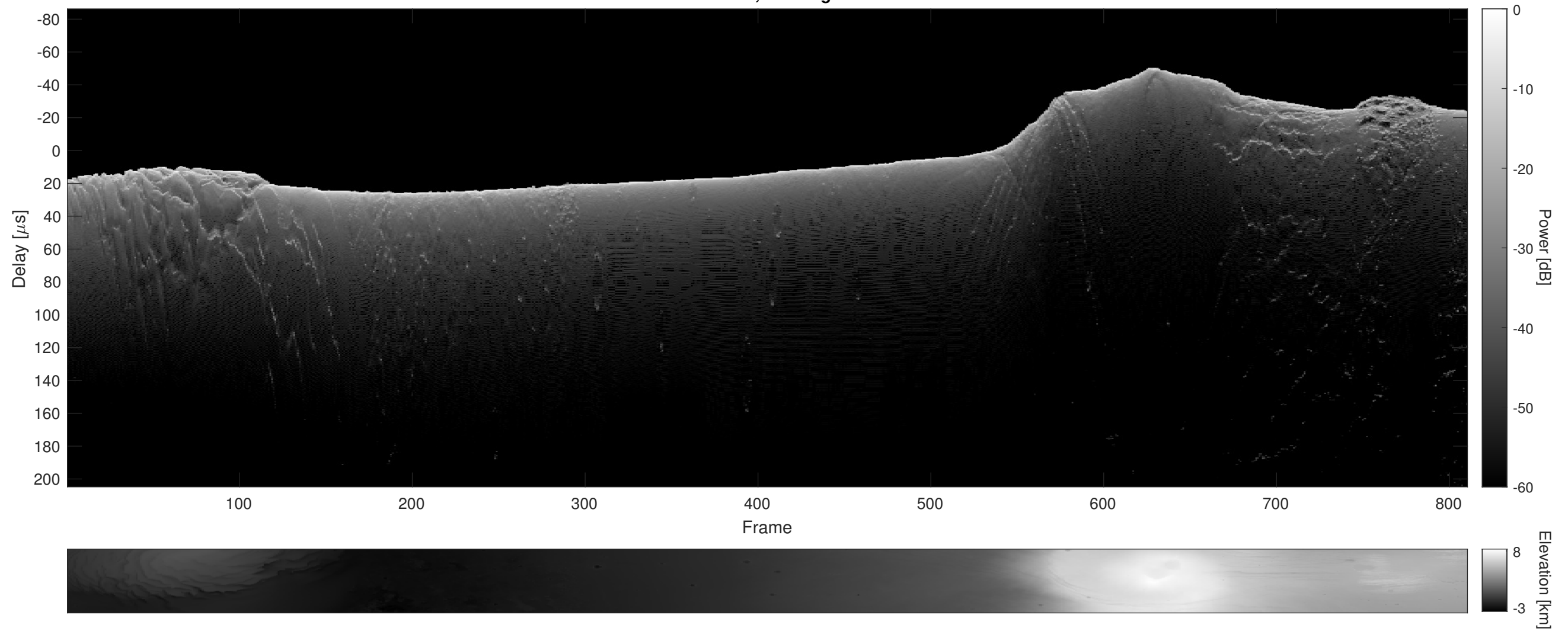
Orbit 9524, Cluttergram
