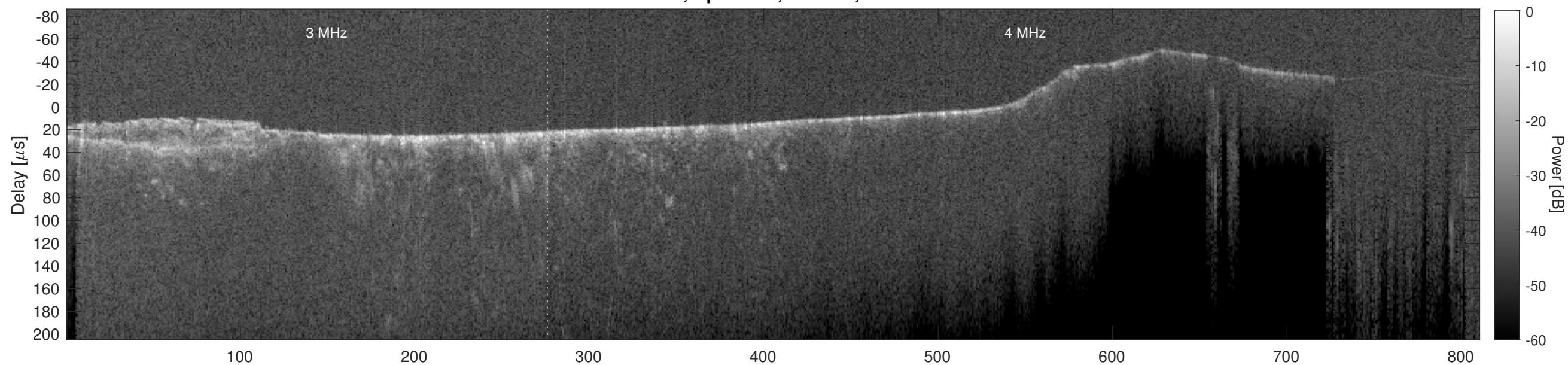
Orbit 9524, Cluttergram
