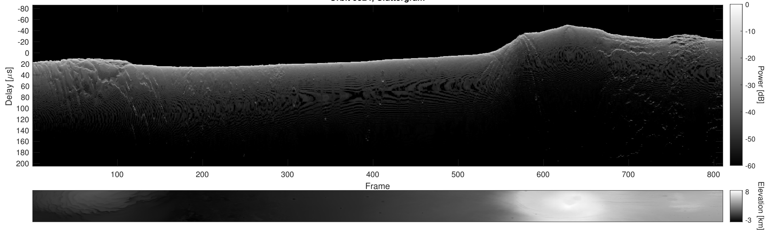
Orbit 9524, Cluttergram
