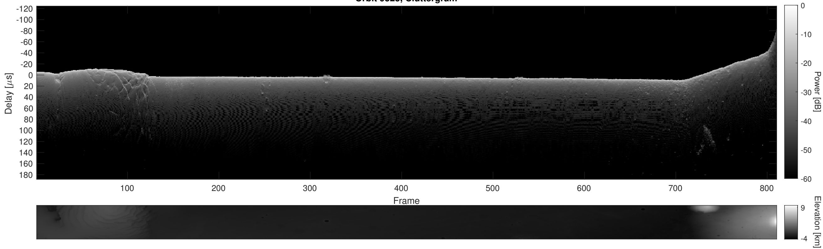
Orbit 9525, Cluttergram
