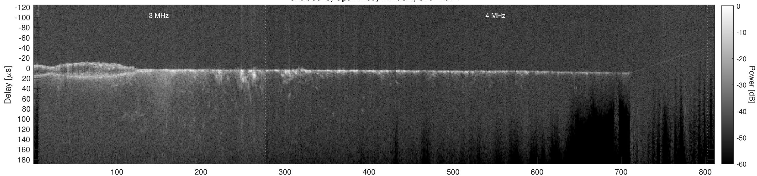
Orbit 9525, Cluttergram
