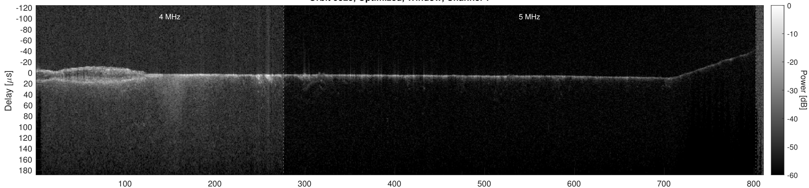
Orbit 9525, Optimized, Window, Channel 2
