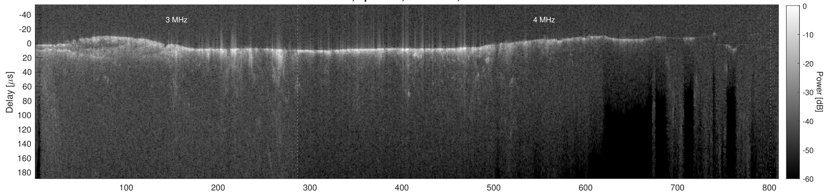
Orbit 9527, Cluttergram
