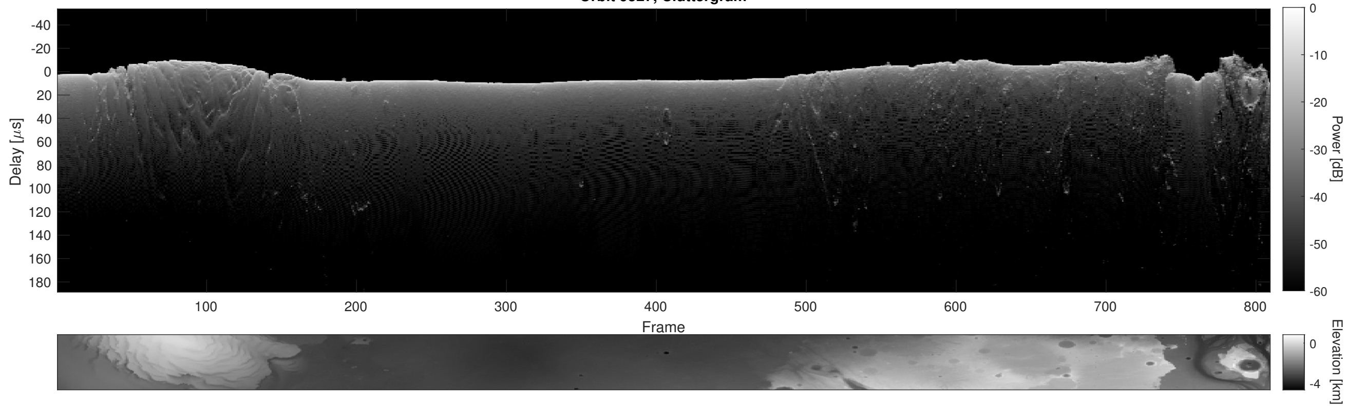
Orbit 9527, Cluttergram
