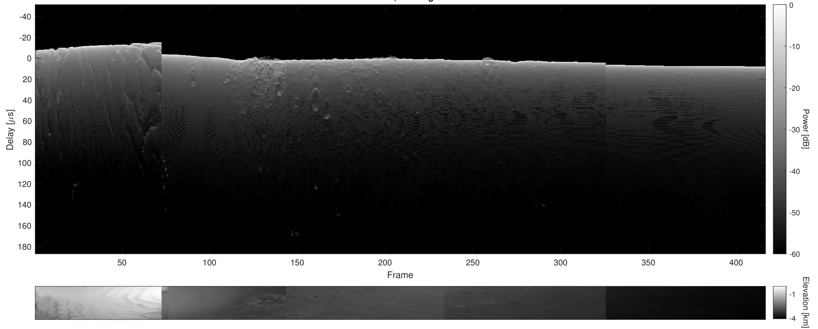
Orbit 9528, Cluttergram
