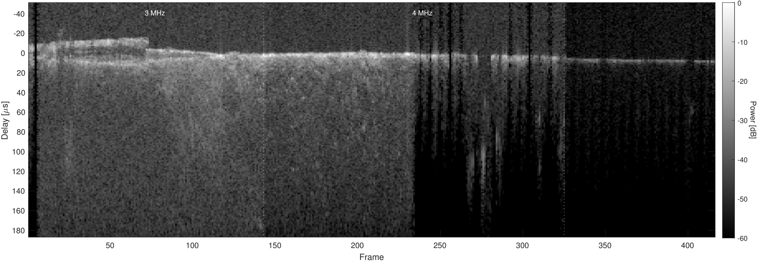
Orbit 9528, Optimized, Window, Channel 2
