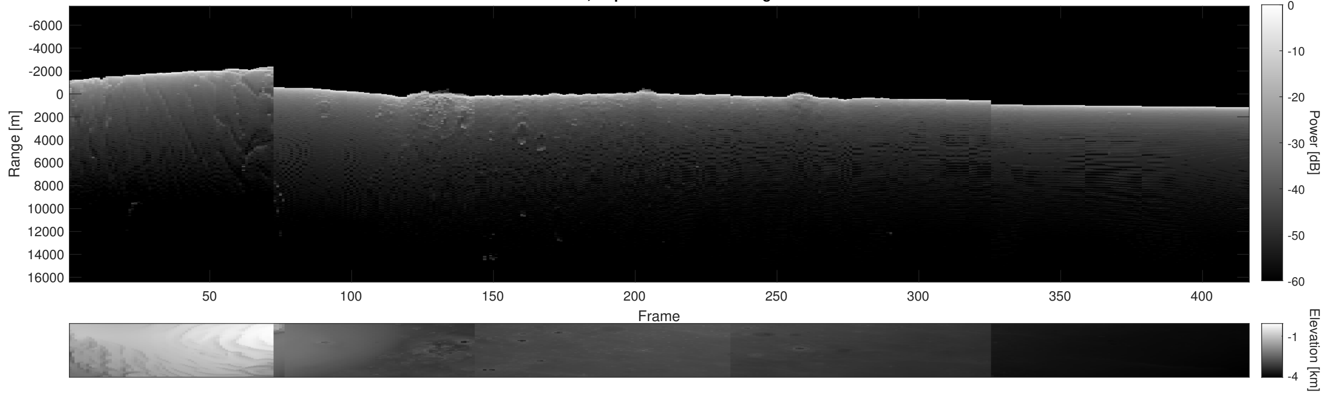
Orbit 9528, Depth-Corrected Cluttergram
