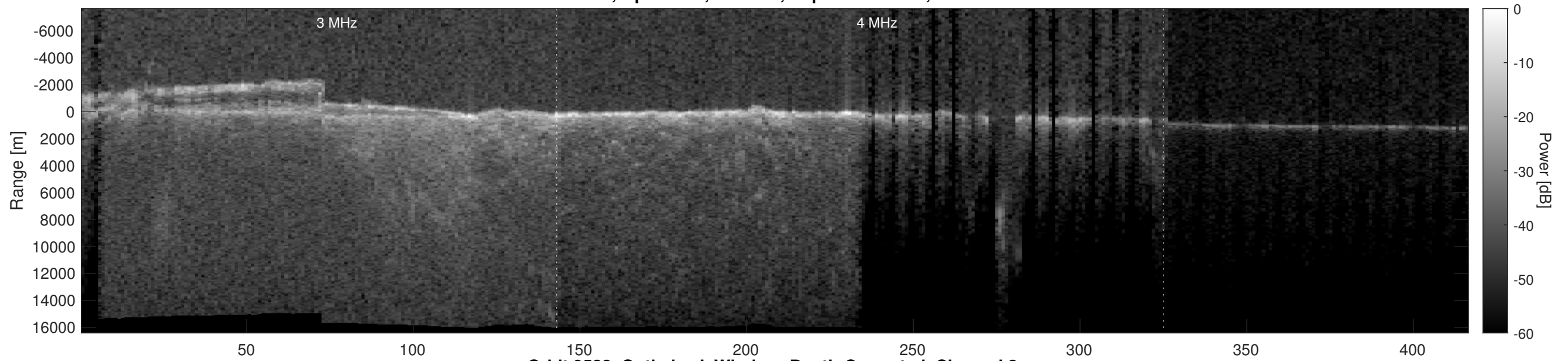
Orbit 9528, Optimized, Window, Depth-Corrected, Channel 2
