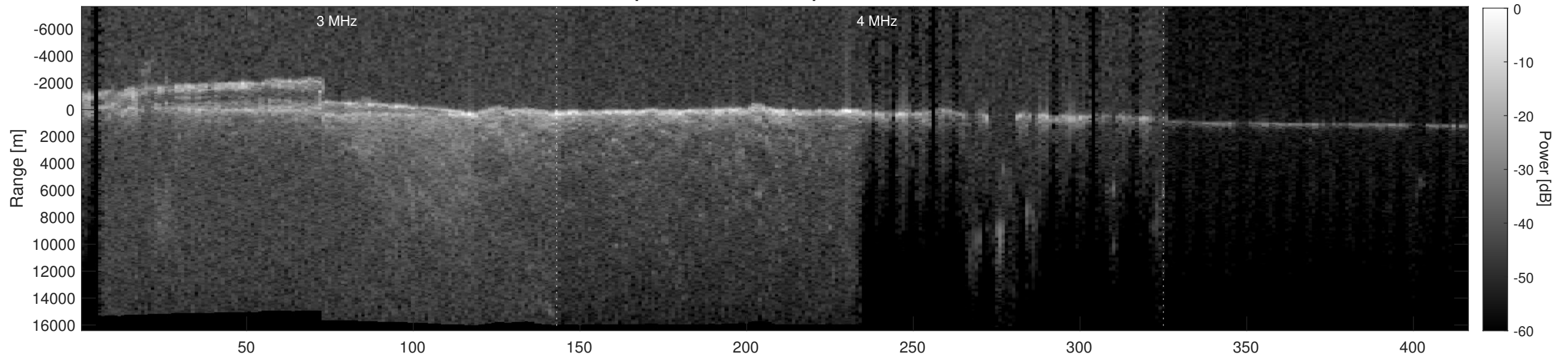
Orbit 9528, Depth-Corrected Cluttergram
