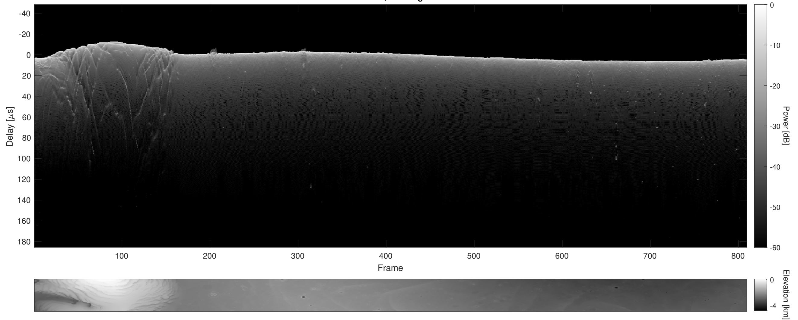
Orbit 9529, Cluttergram
