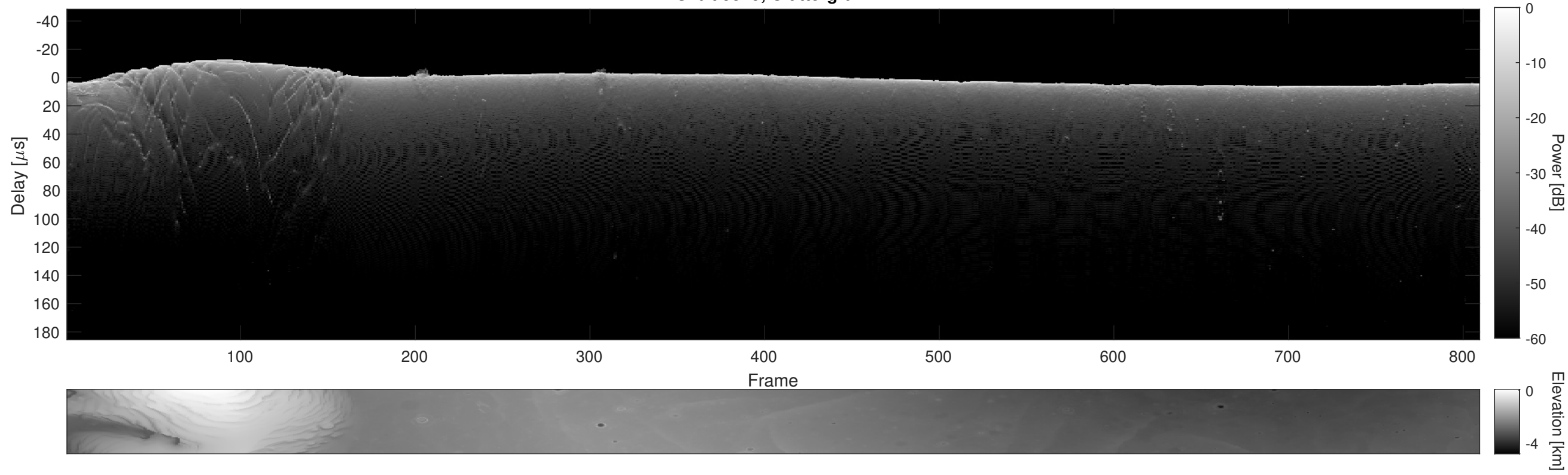
Orbit 9529, Cluttergram
