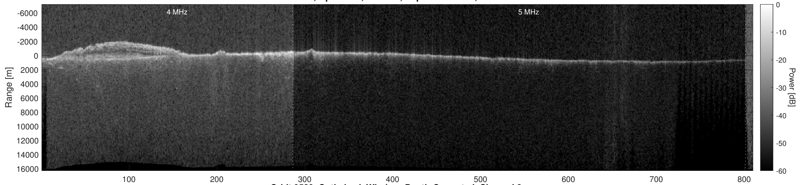
Orbit 9529, Optimized, Window, Depth-Corrected, Channel 2
