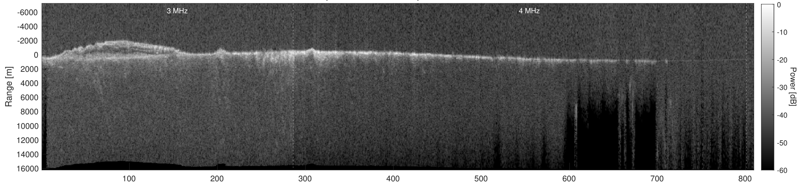
Orbit 9529, Depth-Corrected Cluttergram
