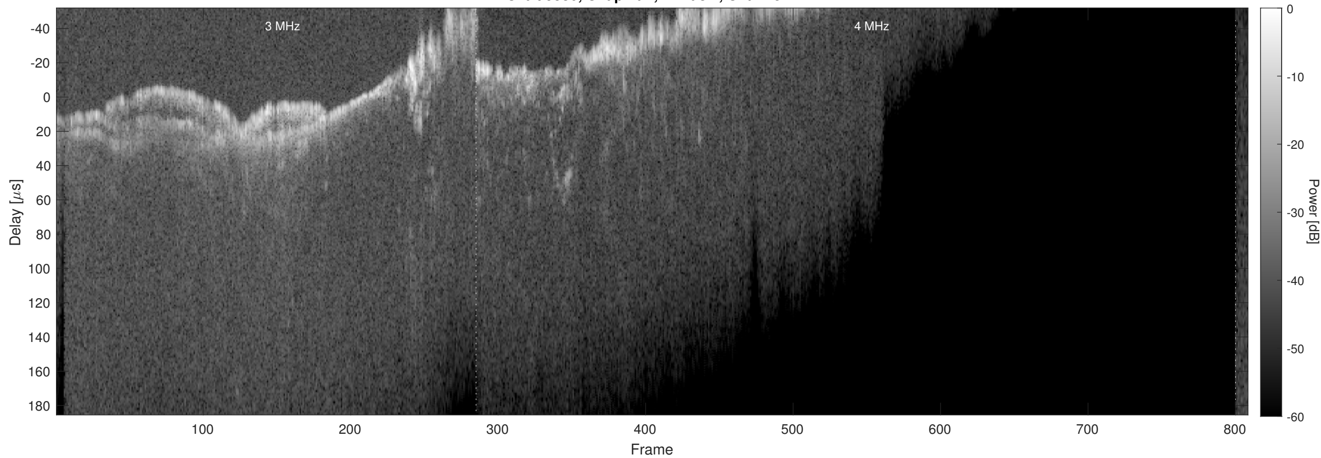
Orbit 9530, Chapman, Window, Channel 2
