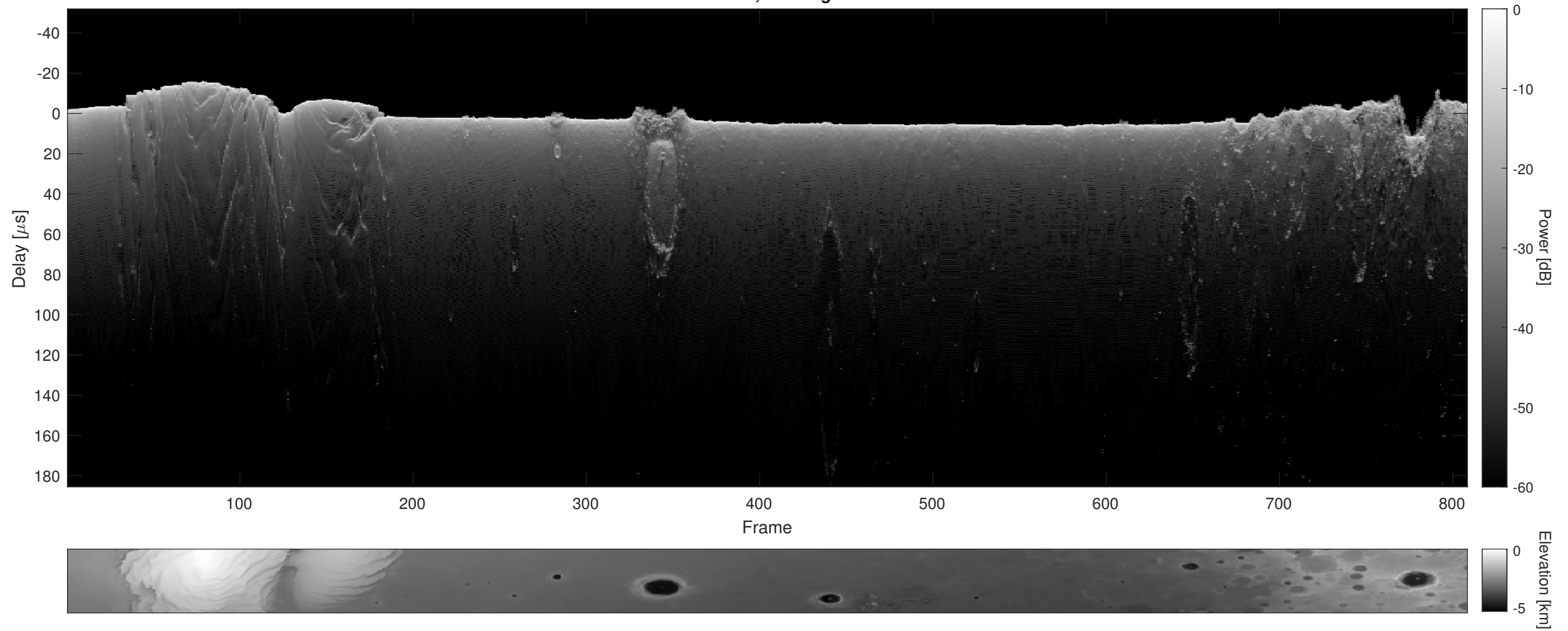
Orbit 9530, Cluttergram
