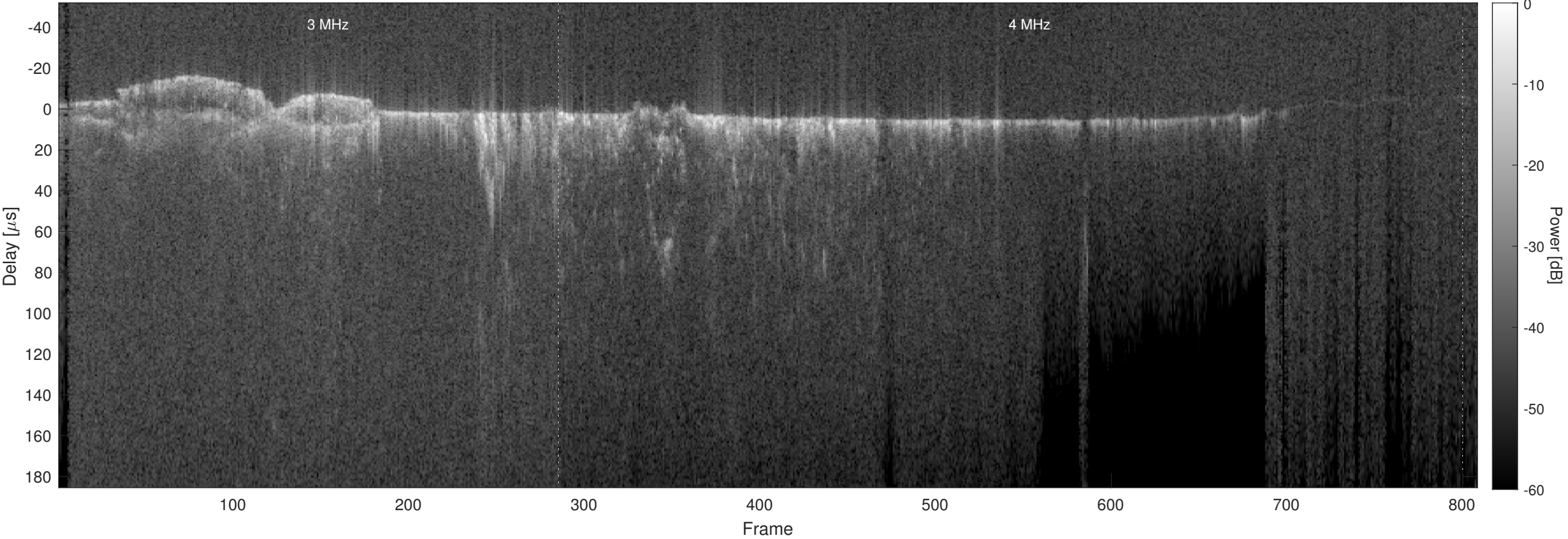
Orbit 9530, Optimized, No Window, Channel 2
