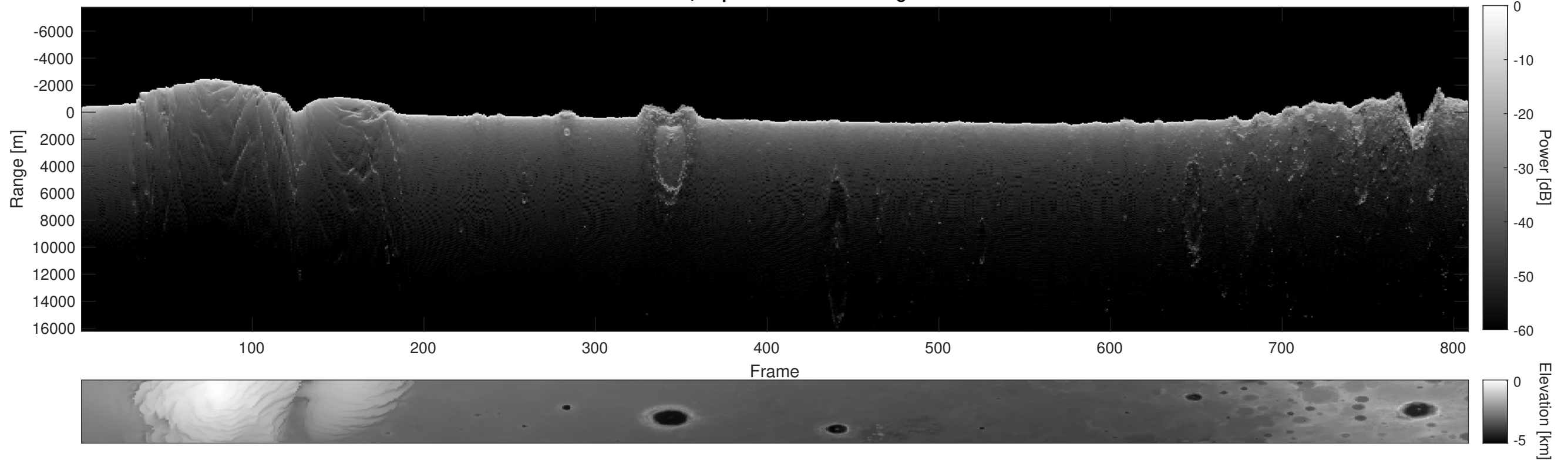
Orbit 9530, Depth-Corrected Cluttergram
