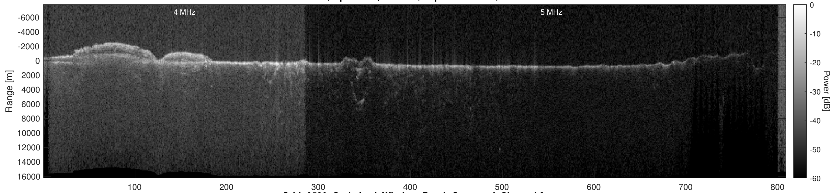
Orbit 9530, Optimized, Window, Depth-Corrected, Channel 2
