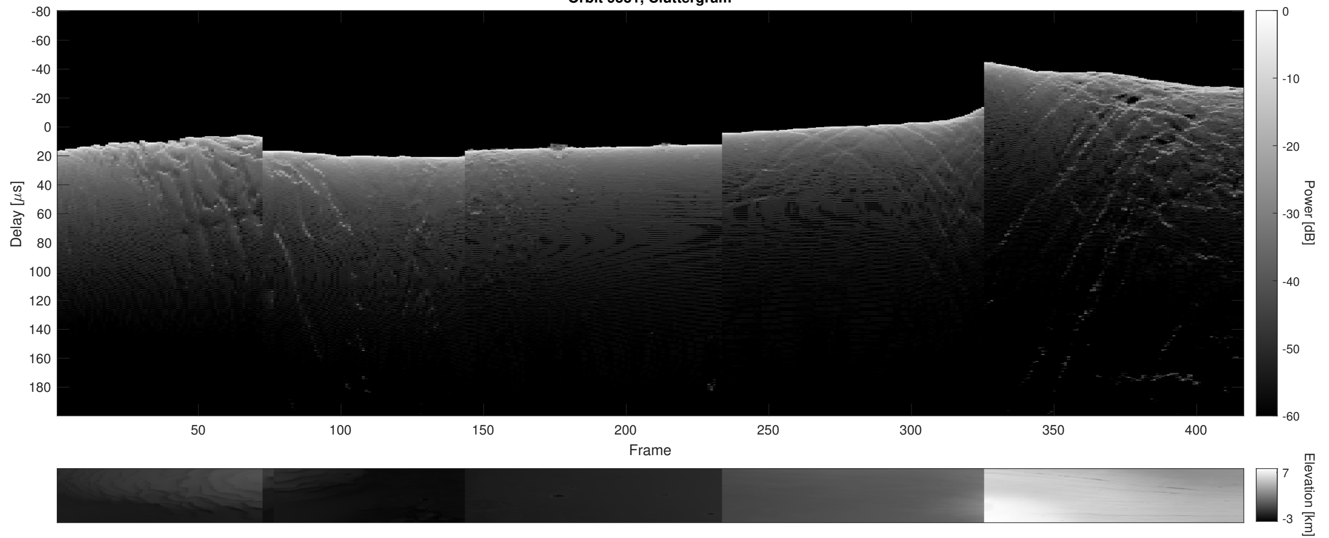
Orbit 9531, Cluttergram
