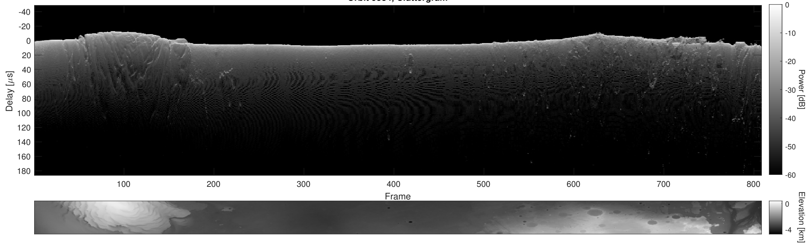
Orbit 9534, Cluttergram
