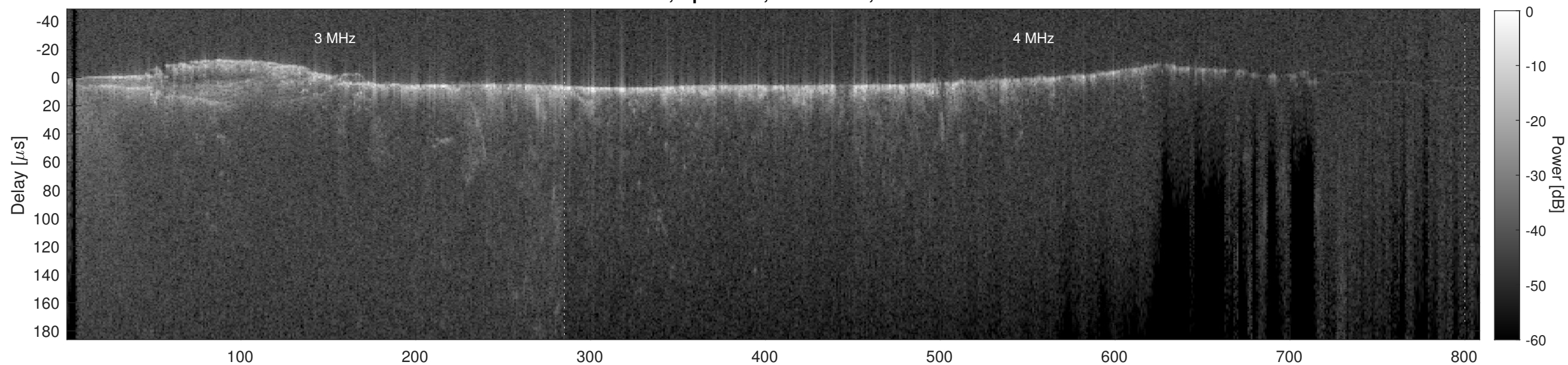
Orbit 9534, Cluttergram
