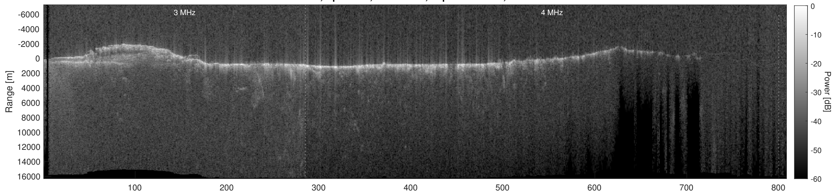
Orbit 9534, Depth-Corrected Cluttergram
