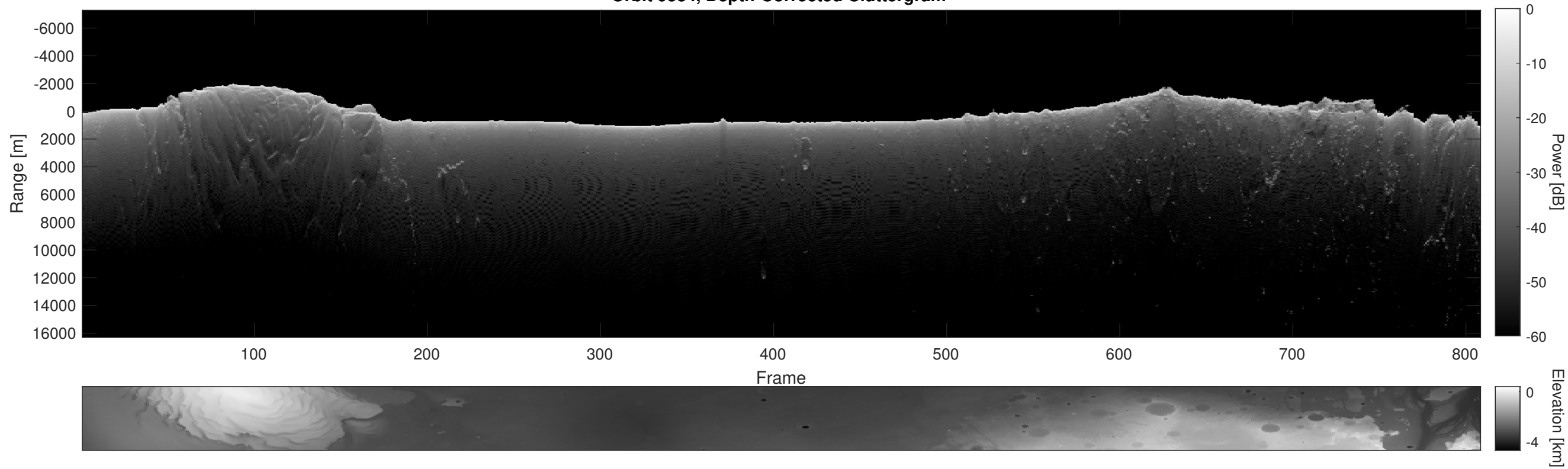
Orbit 9534, Depth-Corrected Cluttergram
