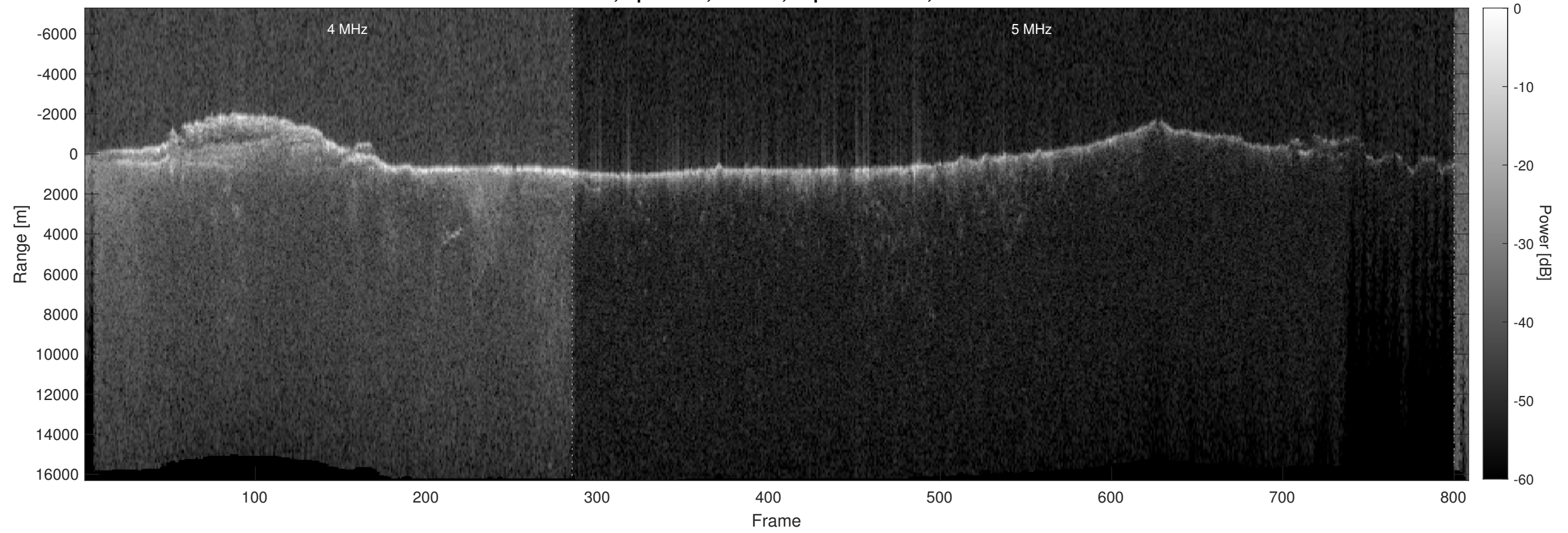
Orbit 9534, Optimized, Window, Depth-Corrected, Channel 2
